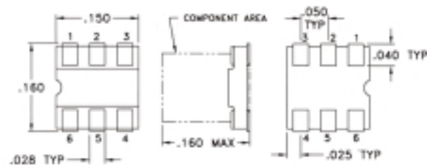
CASE STYLE DRAWINGS & DIMENSIONS (INCH) CASE STYLE DB714
